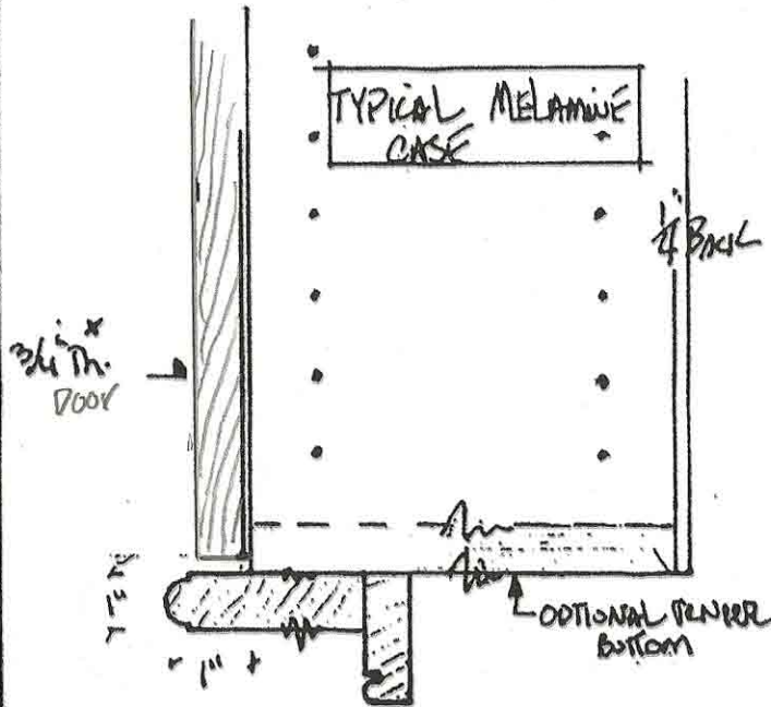
TOP CABINET - SECTION - LIGHT MOLDING EXTENDED
