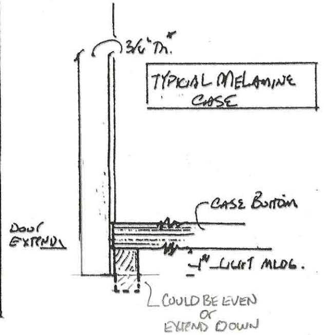
TOP CABINET - SECTION LIGHT MOLDING RECESSED & DOOR EXTENDED
